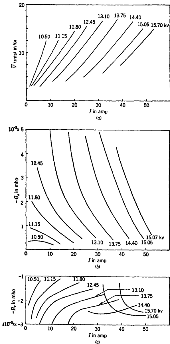
FIG. 7-26.—Plots of (a) rms a-c voltage \bar{V} , (b) electronic conductance G_e , and (c) electronic susceptance B_e , as functions of the input d-c current I , with the input d-c voltage V as parameter.
